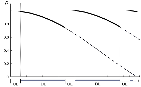
Fig. 2. Evolution of the correlation coefficient between the CSI and the actual channel.
