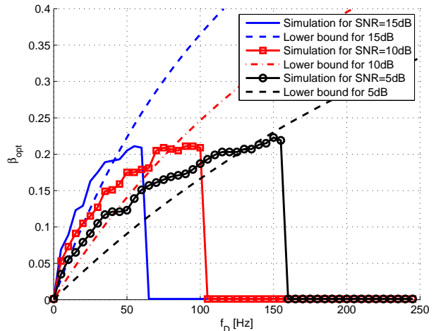
Fig. 5. The optimal fraction of time \beta^{opt} against the mobility of the users.
