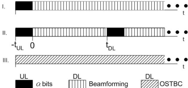
Fig. 4. Proposed scheme: I. No motion: feedback once then use beamforming; II. Small motion: increase rate of feedback, and use beamforming; III. Fast motion: no feedback and OSTBC.
